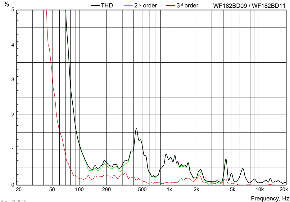
Harmonic Distortion
